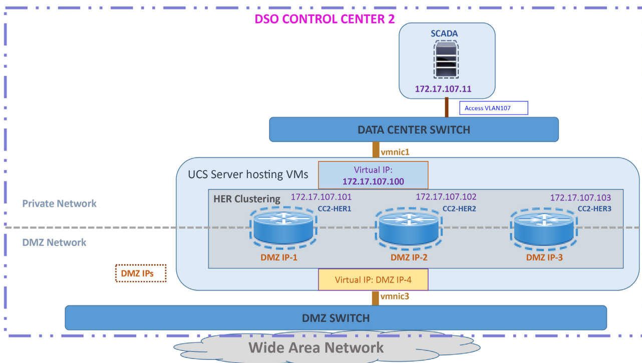
Figure 5 DSO Control Center 2—Implementation Topology
