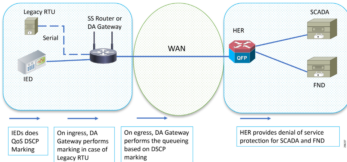
Figure 169 Upstream QoS IED to SCADA
