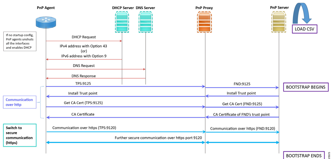
Figure 11 DHCP Server-Assisted Bootstrapping of IoT Gateways—Logical Call Flow
