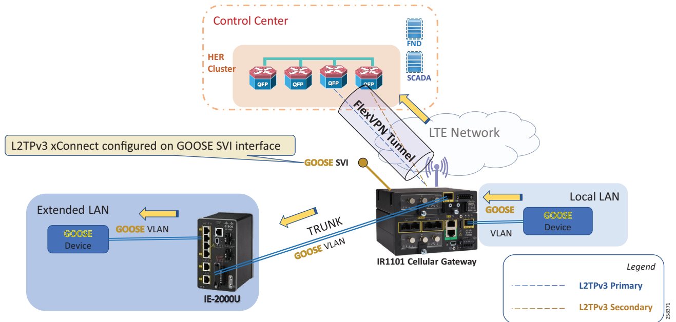
Figure 117 IED-IED GOOSE Architectural Flow
