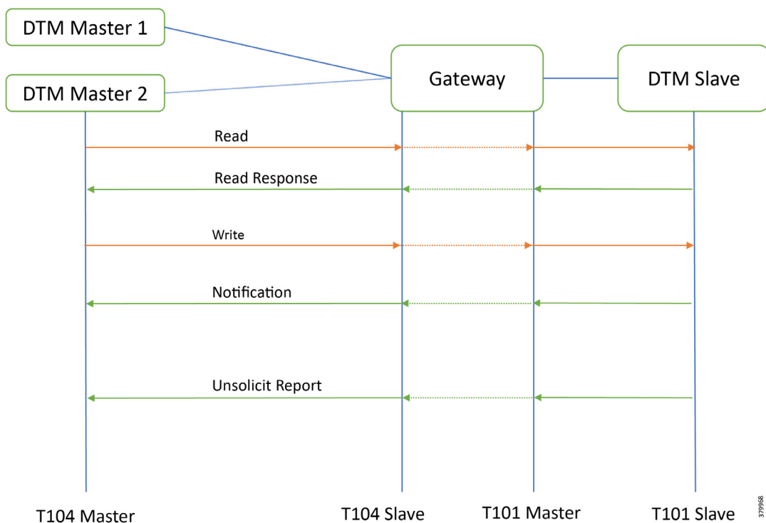
Figure 100 T101 to T104 Protocol Translation Control Flow
