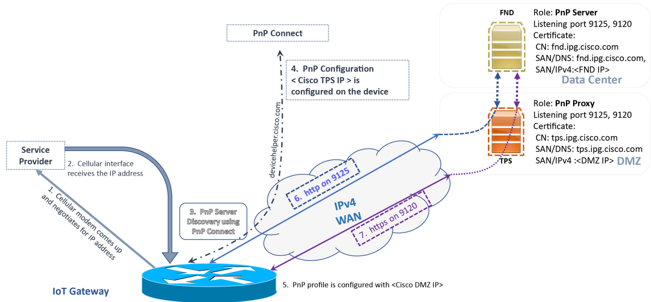
Figure 18 PnP Connect—Assisted Bootstrapping of IoT Gateways
