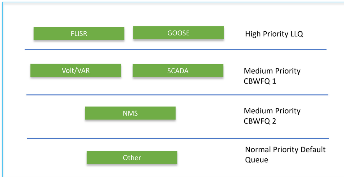
Figure 168 DA Traffic Priority Chart
