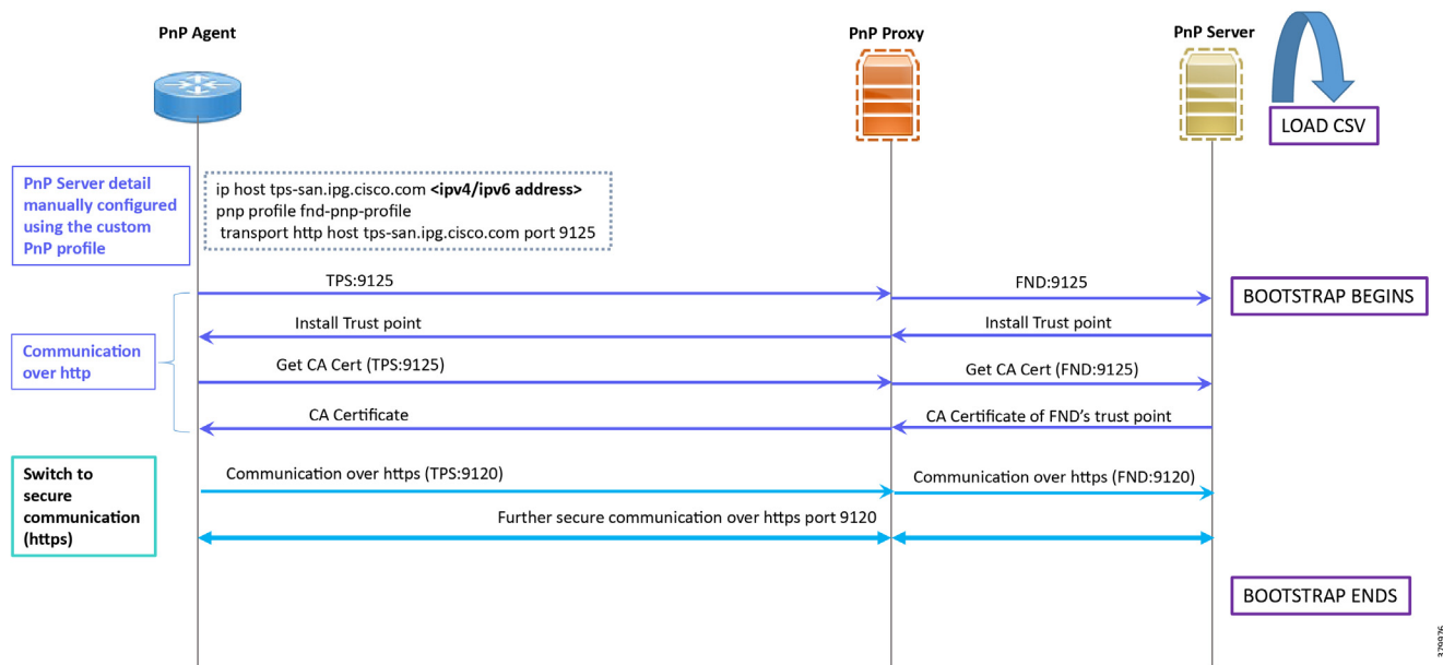
Figure 14 Custom PnP Profile–Assisted Bootstrapping of IoT Gateways—Logical Call Flow
