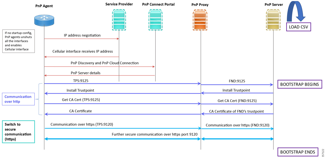
Figure 19 PnP Connect–Assisted Bootstrapping of IoT Gateways—Logical Call Flow
