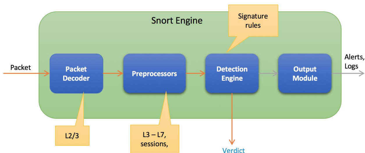
Figure 22. Snort Engine
