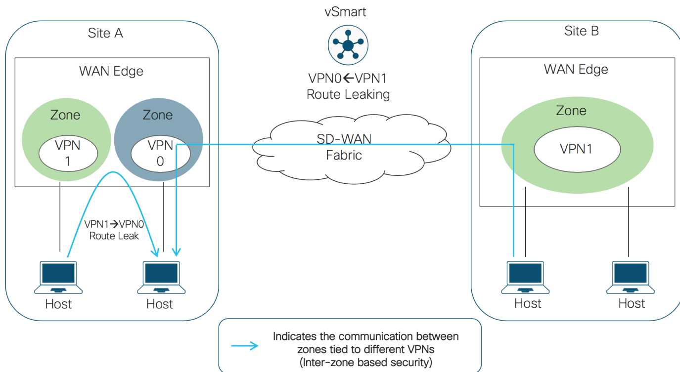
Figure 13. Inter-zone-based security
