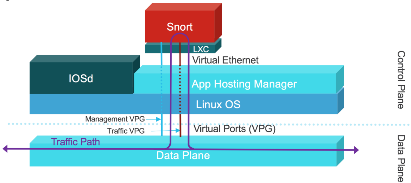
Figure 16. Snort Architecture
