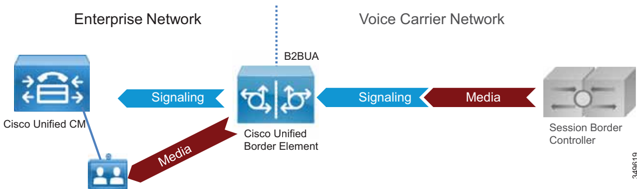
Figure 4-4 Cisco Unified Border Element as B2BUA
