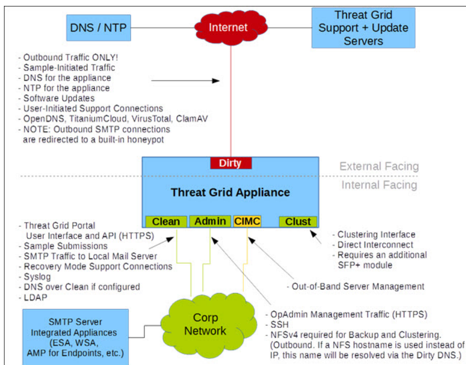
Figure 3: Network Interfaces Setup Diagram
