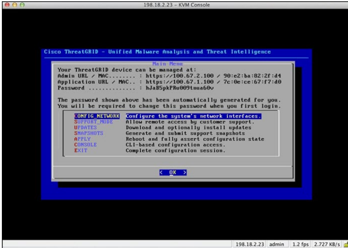
Figure 11: IP Addresses
