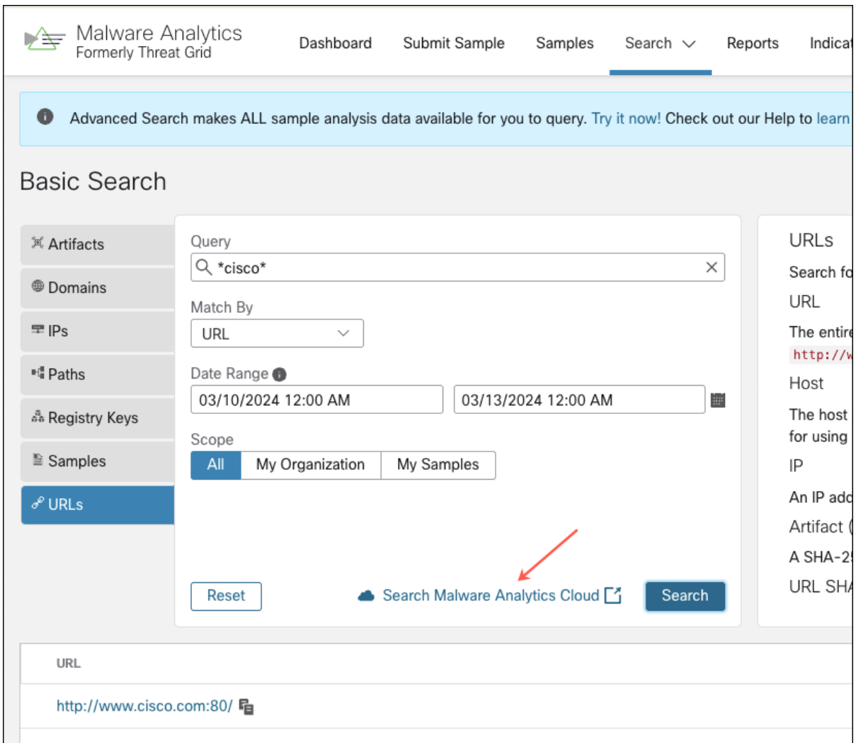
Figure 38: Basic Search - Secure Malware Analytics Cloud link
