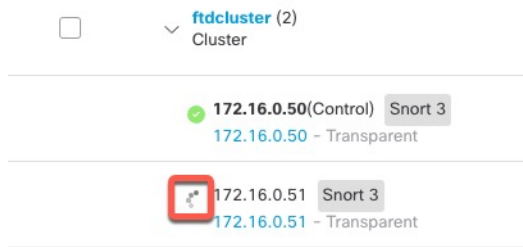
Figure 18: Node Registration
