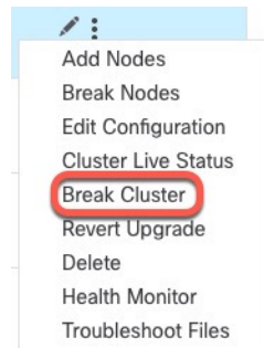
Figure 18: Break Cluster
