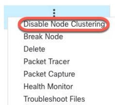
Figure 20: Disable Clustering
