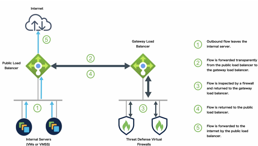
Figure 247: Outbound Traffic Use Case and Topology with GWLB
