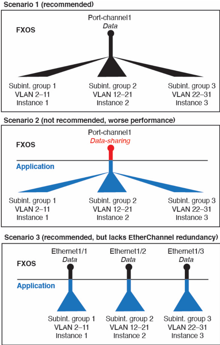
Figure 101: VLANs in the Chassis vs. the Instance
