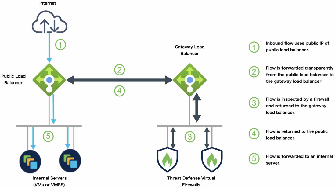
Figure 246: Inbound Traffic Use Case and Topology with GWLB
