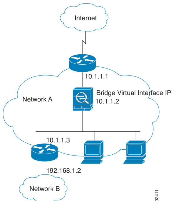
Figure 87: Transparent Firewall Network
