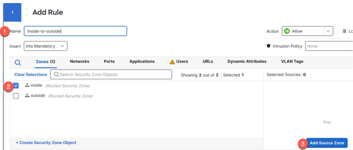
Figure 33: Source Zone
