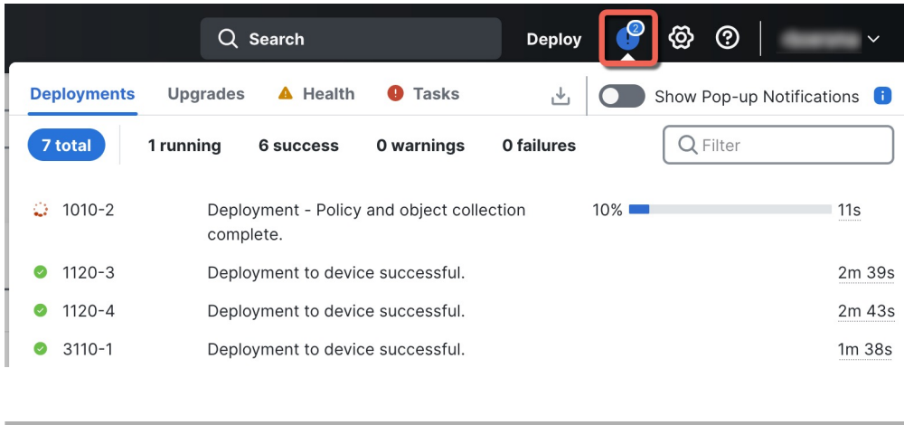
Figure 42: Deployment Status
