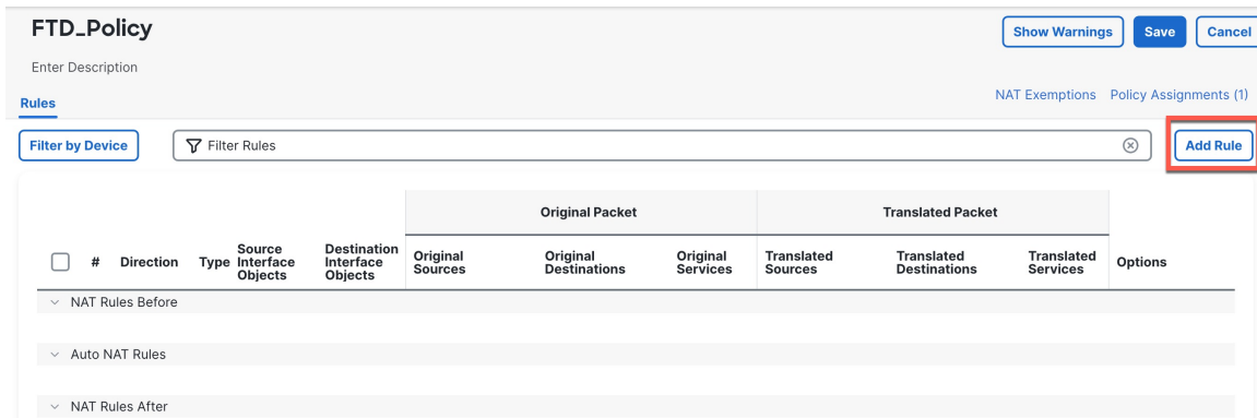
Figure 28: NAT Policy
