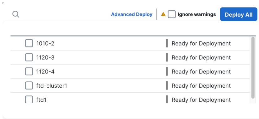
Figure 40: Deploy All
