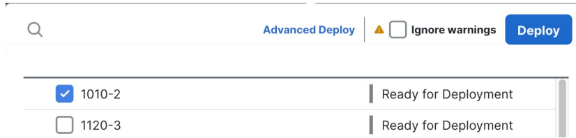
Figure 40: Deploy All
