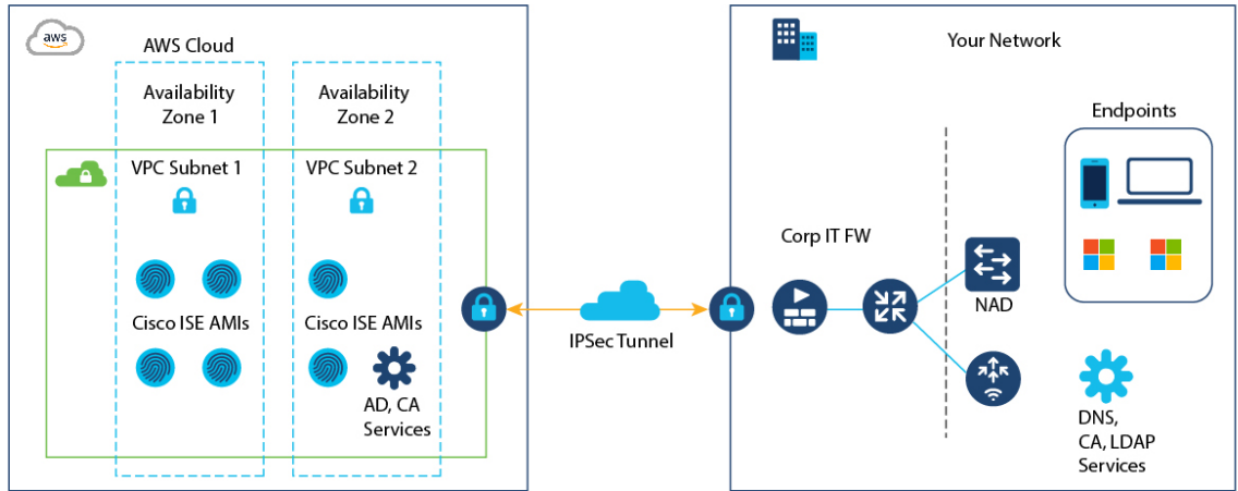
Figure 1: An Example of a Deployment Connected to AWS Cloud
