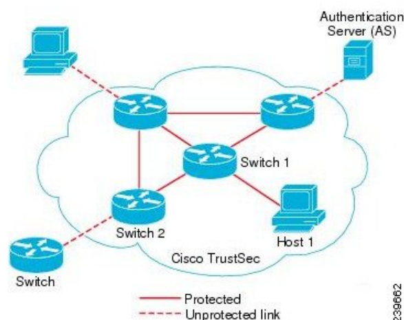
Figure 52: TrustSec Architecture
