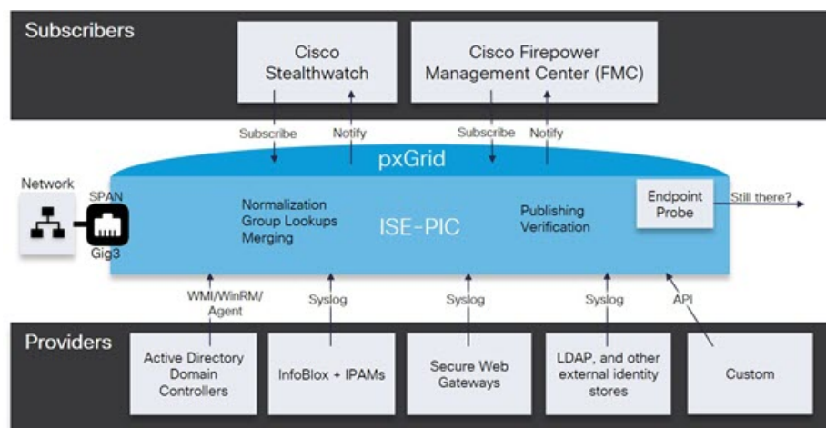
Figure 20: High Level Flow
