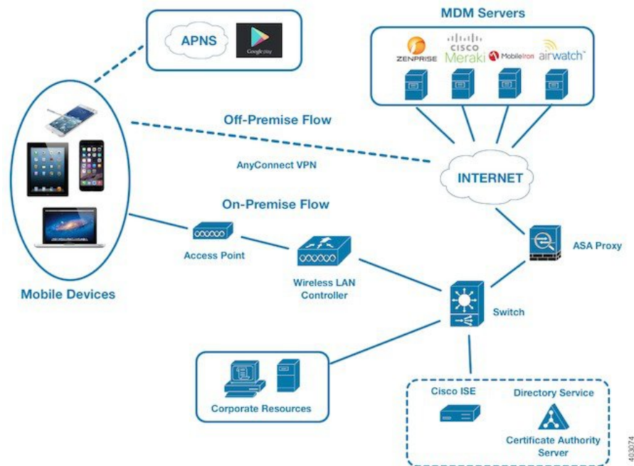
Figure 30: MDM Interoperability with Cisco ISE
