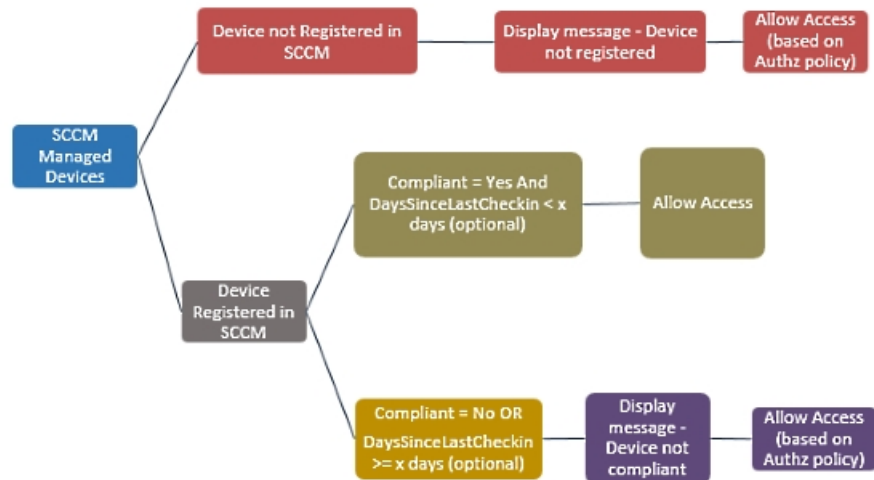
Figure 34: SCCM Workflow
