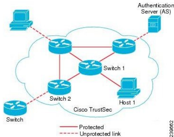
Figure 58: TrustSec Architecture
