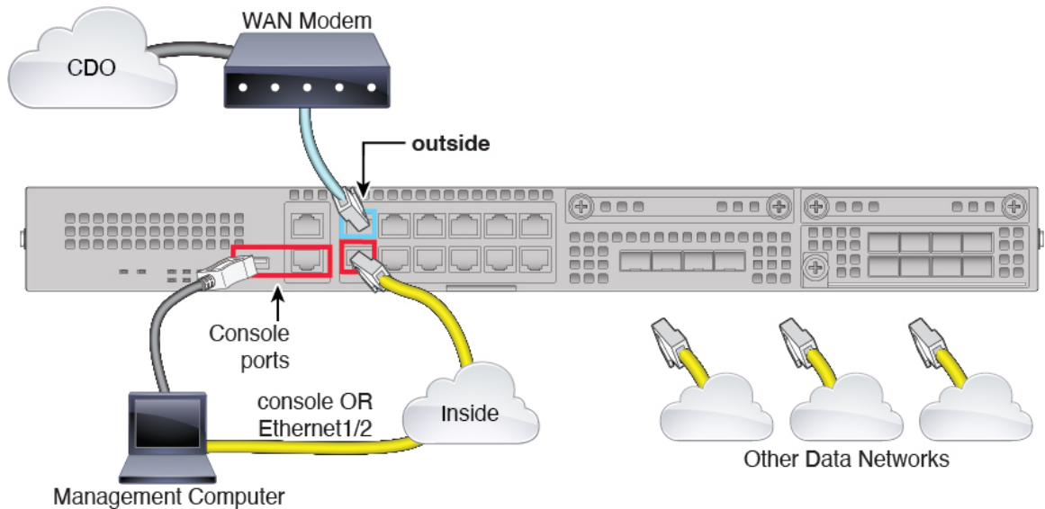
Figure 13: Cabling the Firepower 2100
