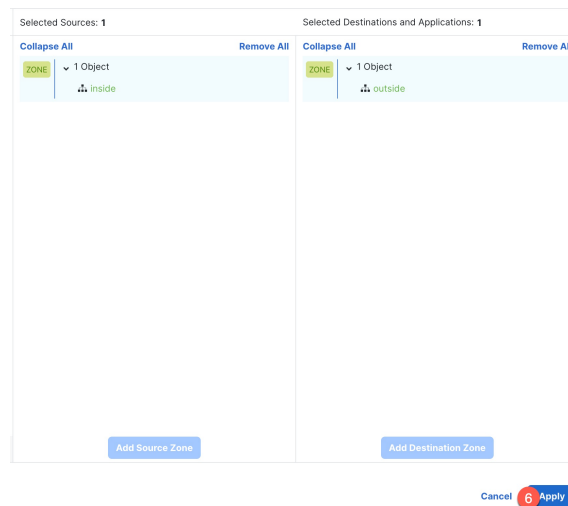
Figure 39: Apply
