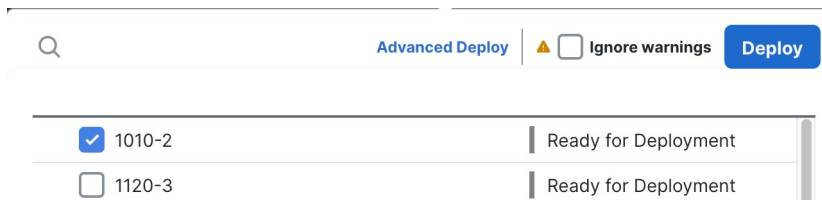
Figure 42: Deploy All
