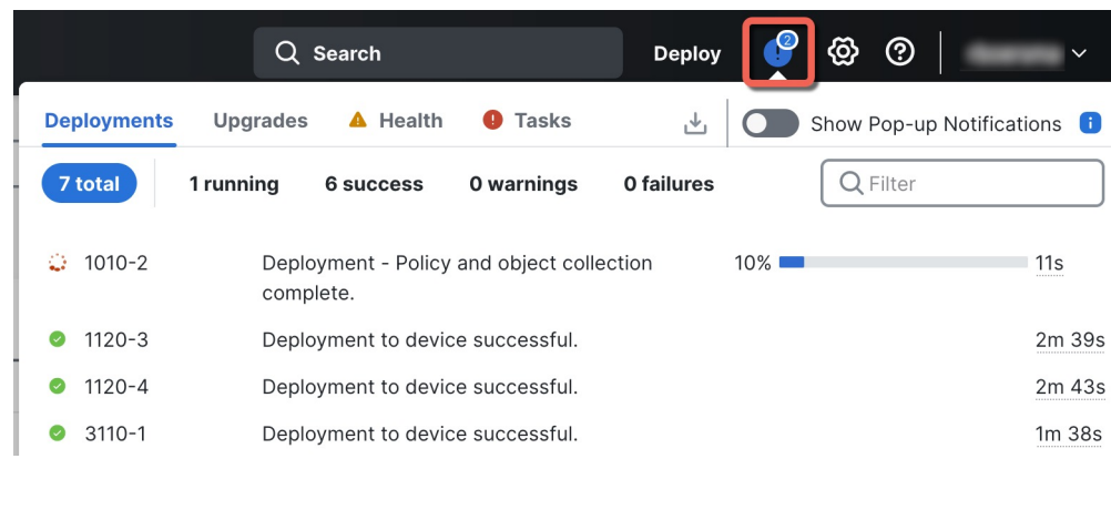
Figure 44: Deployment Status
