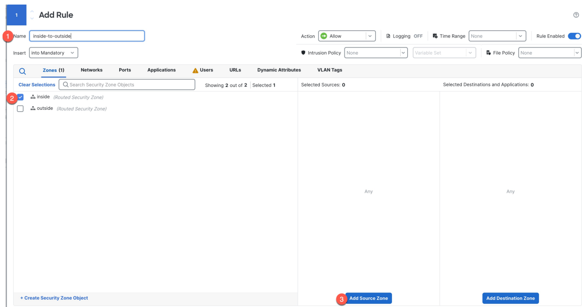
Figure 37: Source Zone
