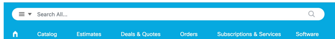
Figure 3: License Search
