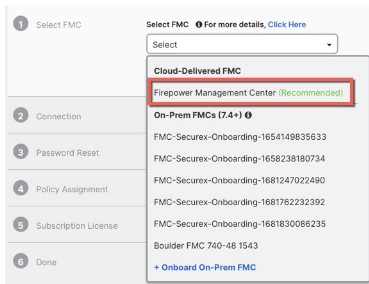
Figure 7: Select FMC
