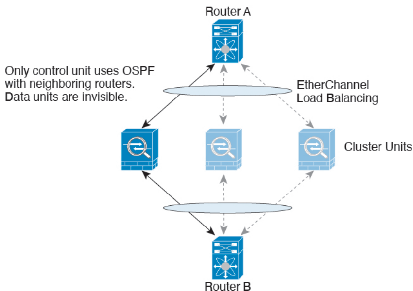
Figure 9: Dynamic Routing
