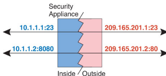
Figure 20: Typical Static NAT with Port Translation Scenario
