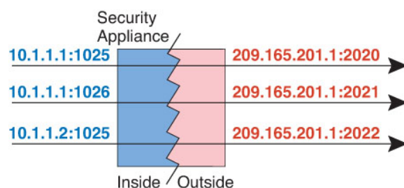
Figure 18: Dynamic PAT
