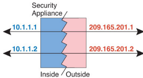
Figure 19: Static NAT
