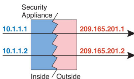
Figure 58: Dynamic NAT
