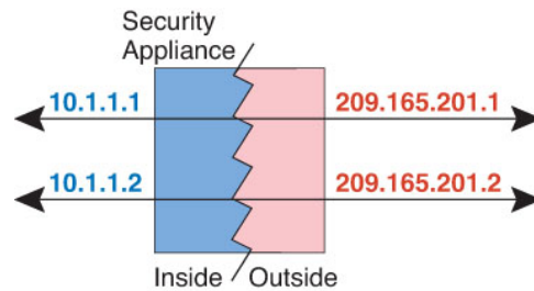
Figure 61: Static NAT
