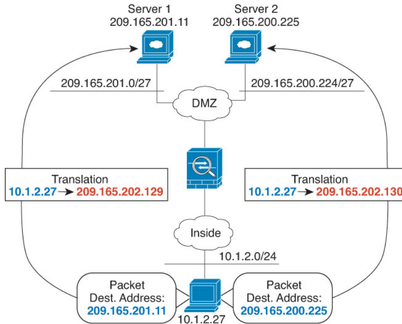
Figure 28: Manual NAT with Different Destination Addresses
