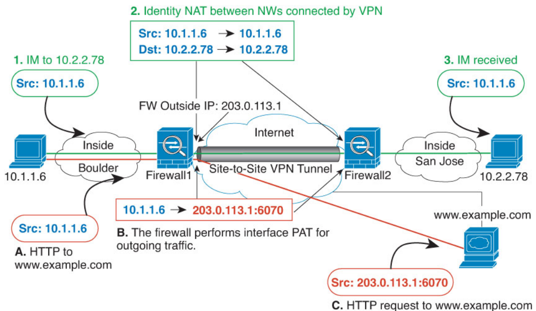
Figure 30: Interface PAT and Identity NAT for Site-to-Site VPN
