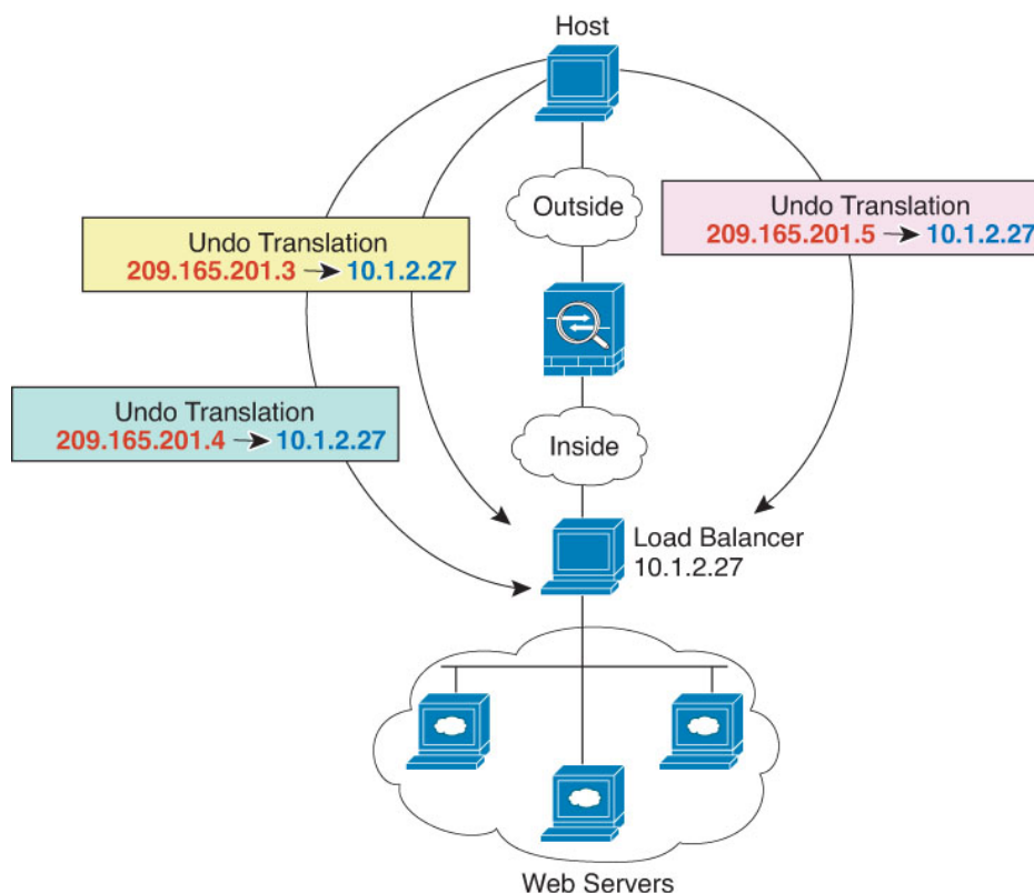
Figure 22: One-to-Many Static NAT Example
