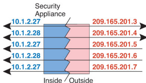
Figure 23: Few-to-Many Static NAT
