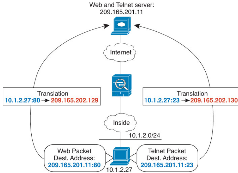
Figure 29: Manual NAT with Different Destination Ports
