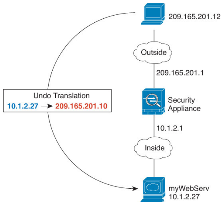
Figure 26: Static NAT for an Inside Web Server
