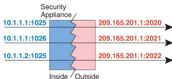
Figure 18: Dynamic PAT
