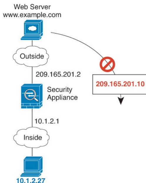
Figure 17: Remote Host Attempts to Initiate a Connection to a Mapped Address
