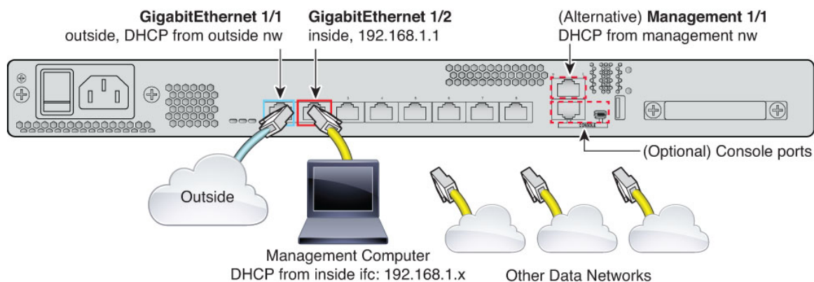
Figure 1: Cabling the ASA 5508-X or 5516-X
