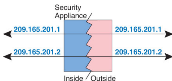
Figure 25: Identity NAT
