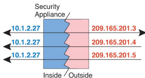
Figure 21: One-to-Many Static NAT
