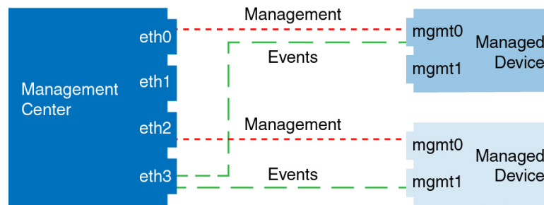
Figure 50: Mixed Management and Event Interface Usage
