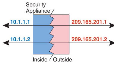
Figure 57: Static NAT
