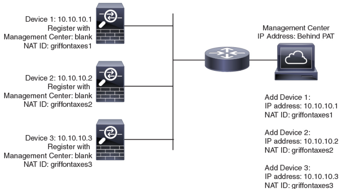
Figure 46: NAT ID for FMC Behind PAT
