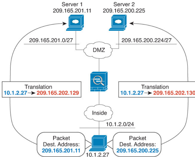
Figure 68: Manual NAT with Different Destination Addresses
