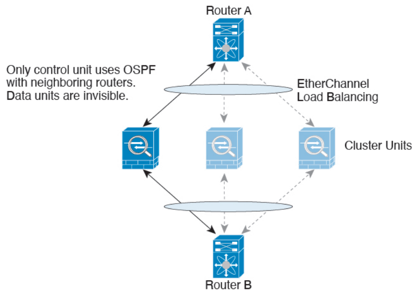
Figure 39: Dynamic Routing
