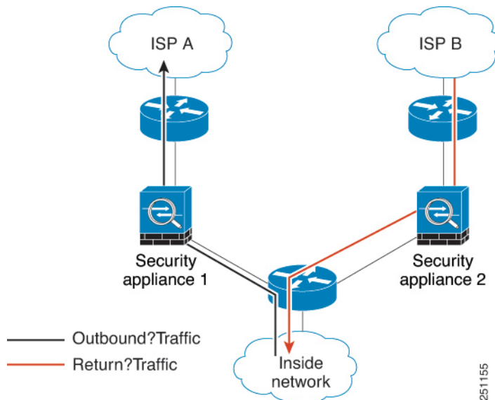
Figure 44: Asymmetric Routing
