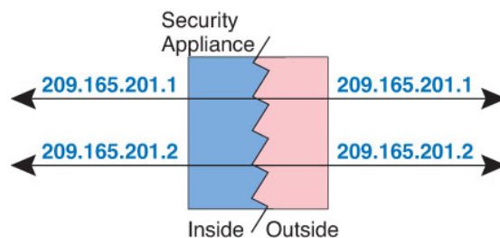
Figure 63: Identity NAT
