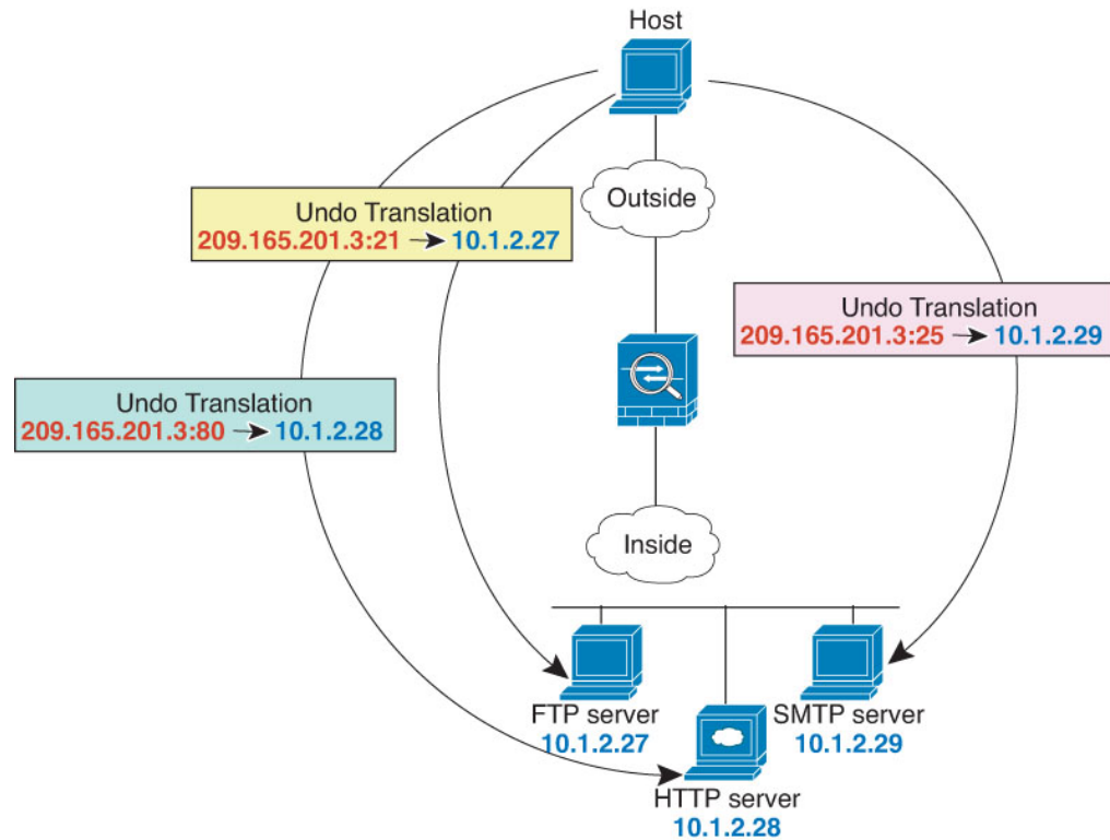
Figure 67: Static NAT-with-Port-Translation
