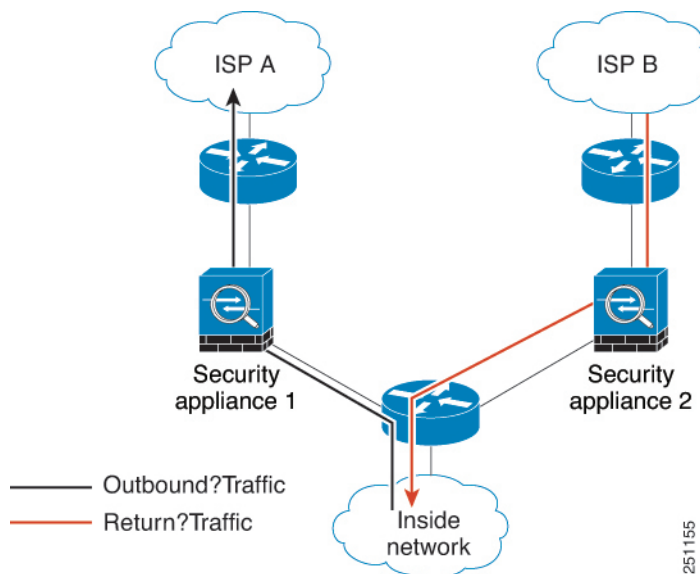
Figure 36: Asymmetric Routing
