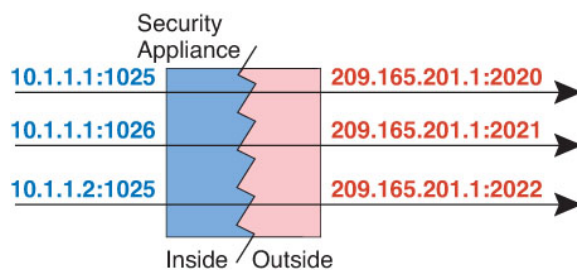
Figure 48: Dynamic PAT
