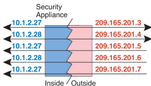
Figure 53: Few-to-Many Static NAT
