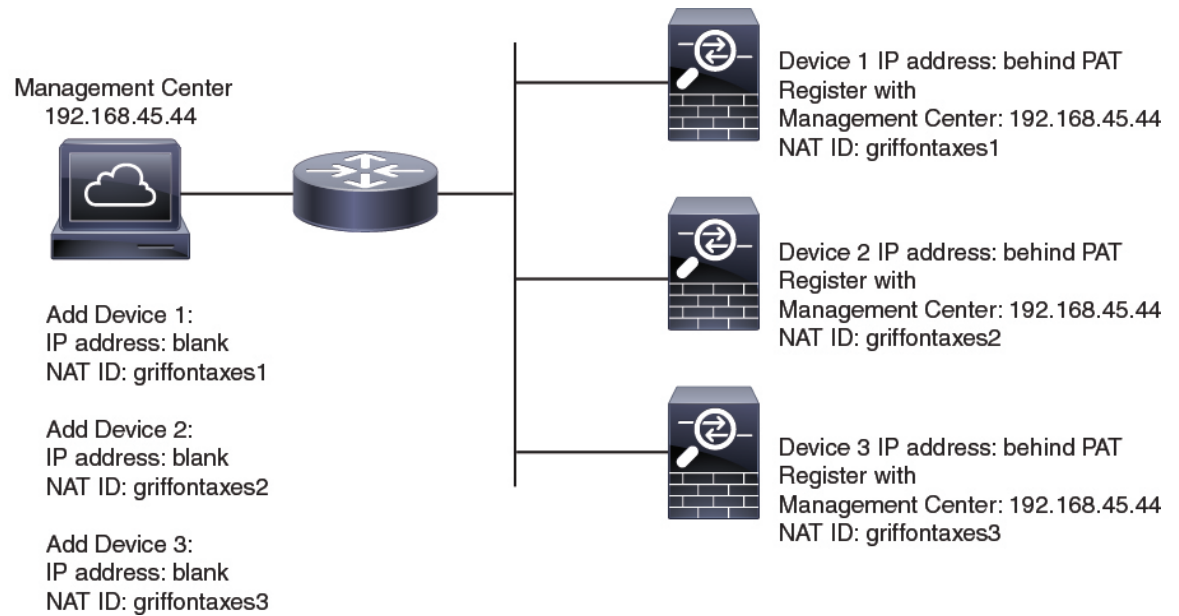
Figure 37: NAT ID for Managed Devices Behind PAT
