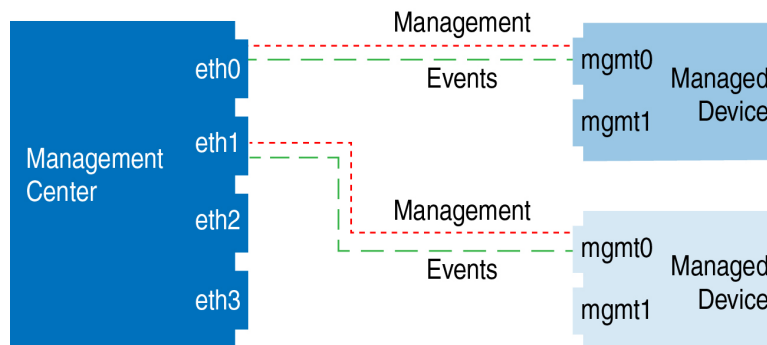
Figure 40: Multiple Management Interfaces on the Firepower Management Center
