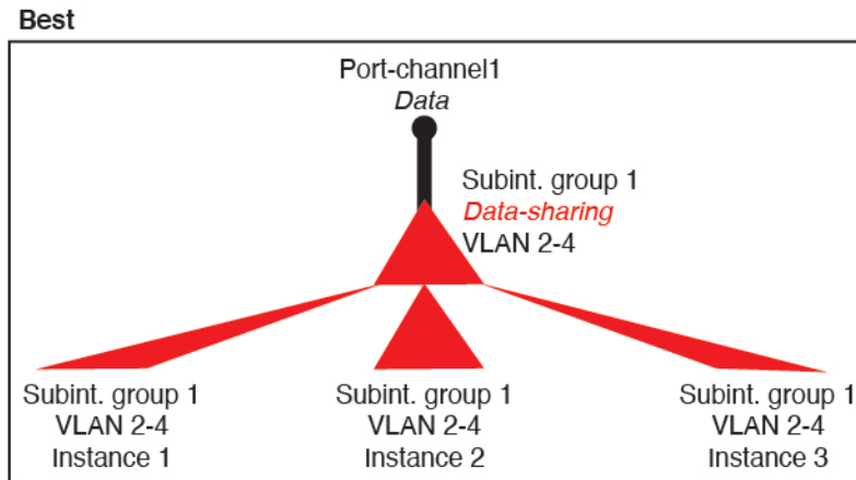
Figure 12: Best: Shared Subinterface Group on One Parent
