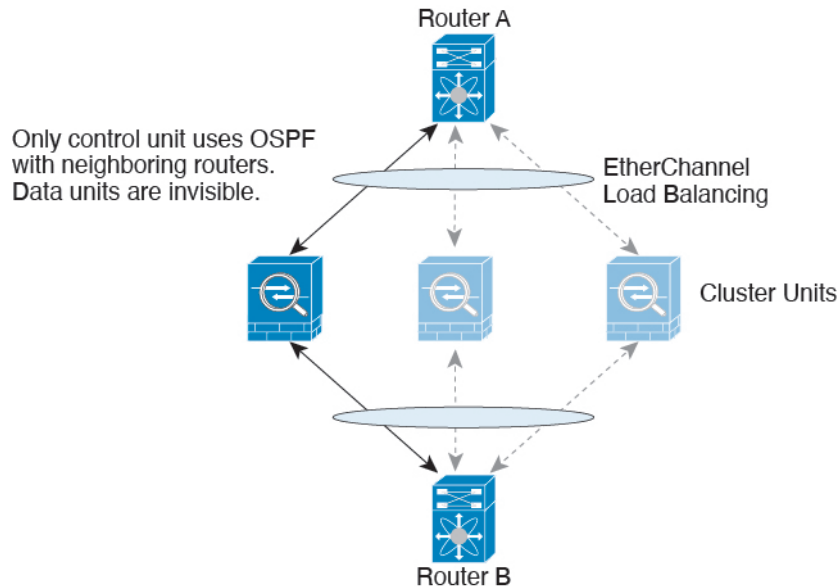
Figure 24: Dynamic Routing
