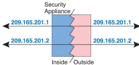
Figure 44: Identity NAT
