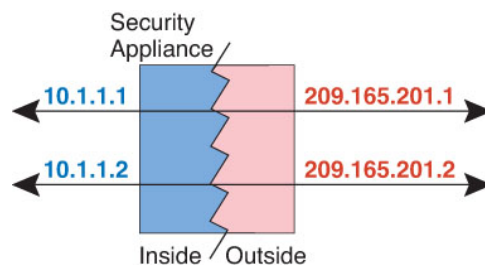
Figure 38: Static NAT
