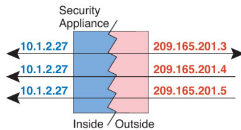
Figure 40: One-to-Many Static NAT
