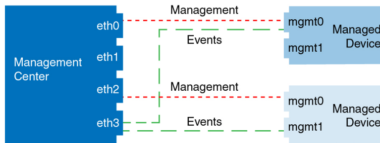
Figure 31: Mixed Management and Event Interface Usage
