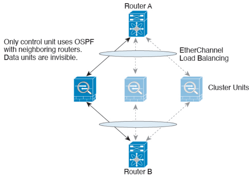
Figure 21: Dynamic Routing
