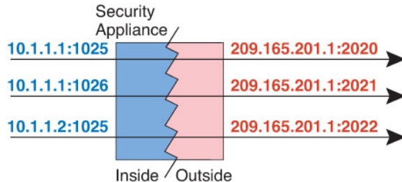
Figure 34: Dynamic PAT
