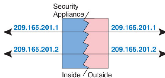
Figure 41: Identity NAT
