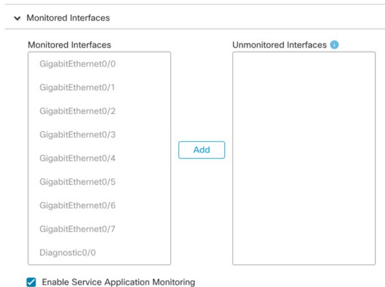
Figure 5: Configure Monitored Interfaces
