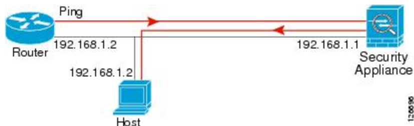
Figure 91: Ping Failure Because of IP Addressing Problems
