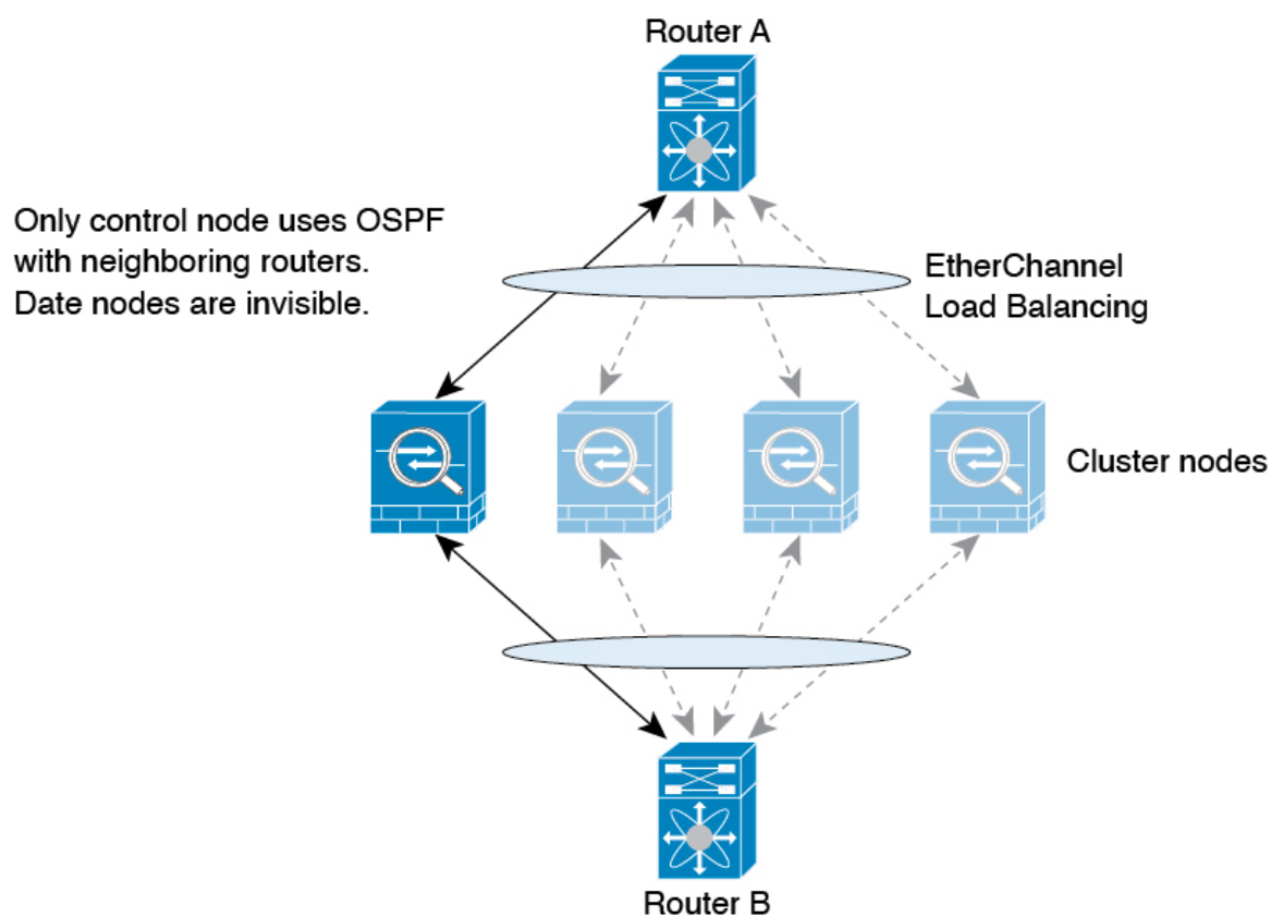
Figure 76: Dynamic Routing in Spanned EtherChannel Mode
