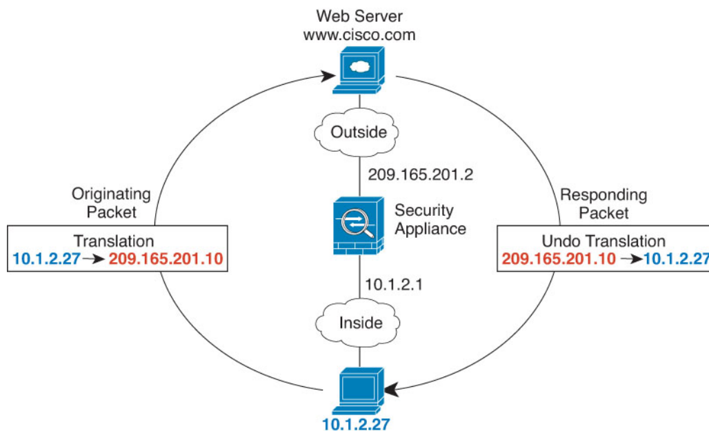
Figure 7: NAT Example: Routed Mode
