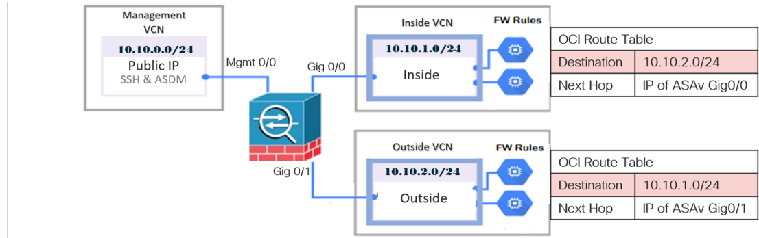
Figure 51: Sample ASAv on OCI Deployment
