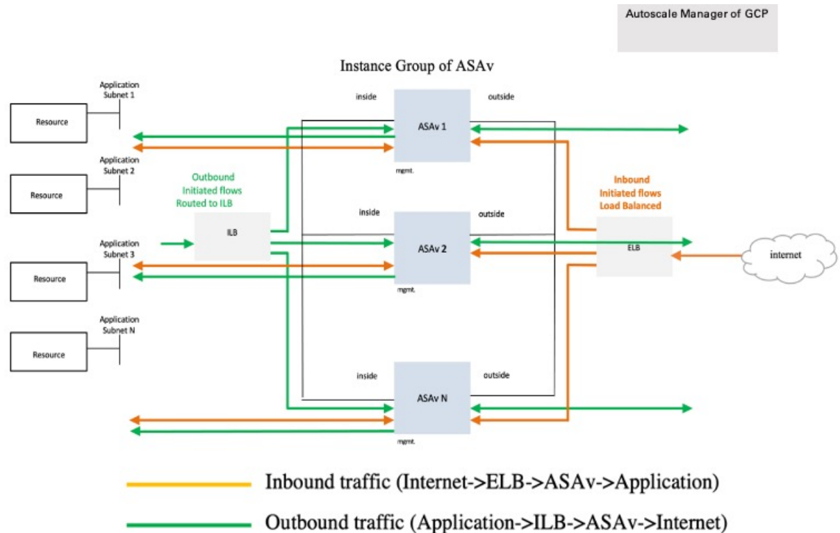
Figure 56: ASAv Auto Scale Use Case
