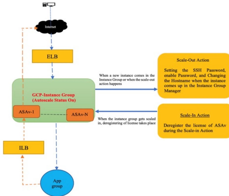
Figure 60: Autoscale Solution Overview
