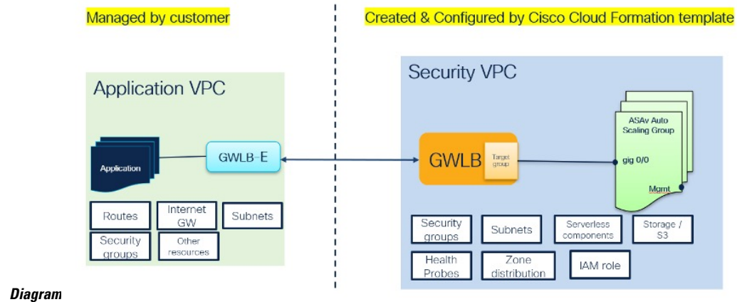
Figure 16: ASAv AWS GWLB Auto Scale Use Case
