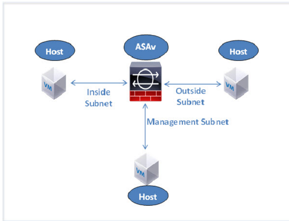
Figure 38: Recommended Topology for the ASAv in Routed Firewall Mode
