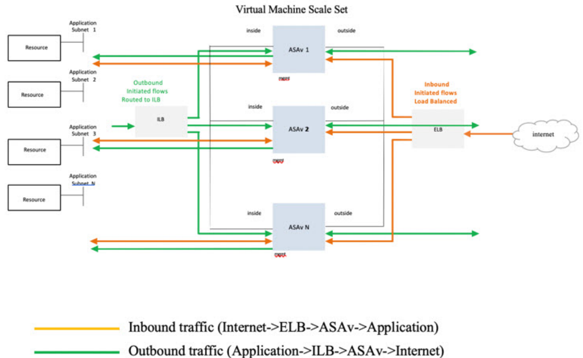
Figure 17: ASAv Auto Scale using Sandwich Topology Use Case
