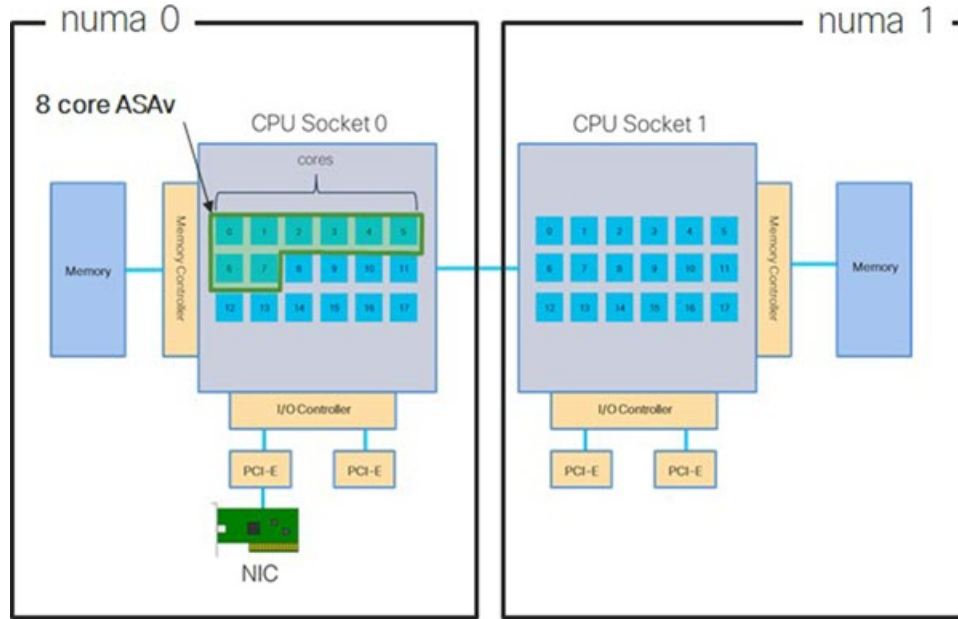
Figure 7: 8-Core ASAv NUMA Architecture Example
