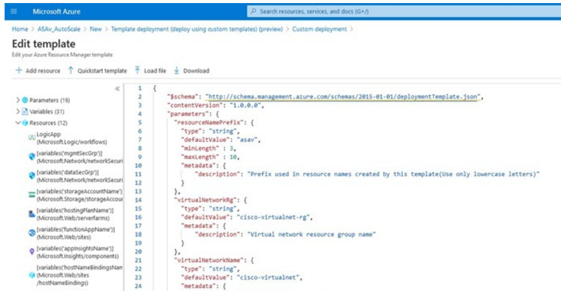
Figure 20: Edit Template
