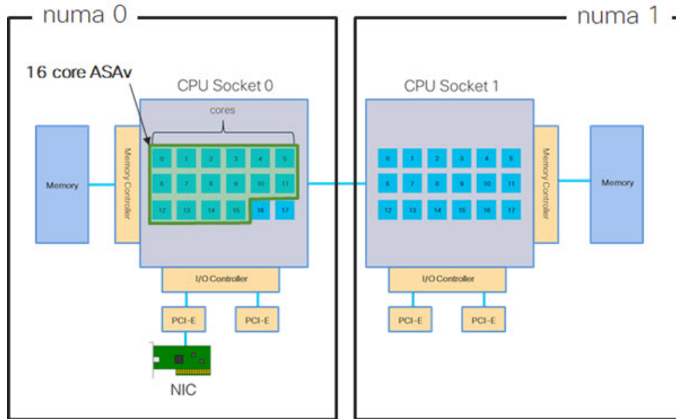
Figure 8: 16-Core ASAv NUMA Architecture Example
