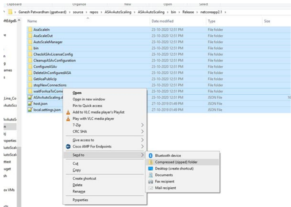
Figure 36: Build ASM_Function.zip
