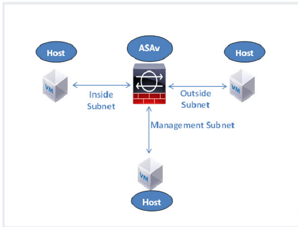
Figure 11: Recommended Topology for the ASAv in Routed Firewall Mode
