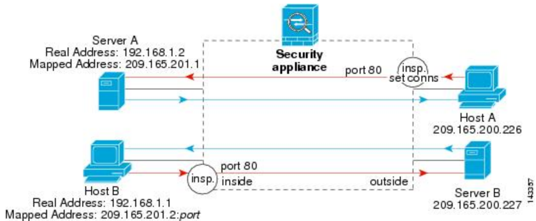
Figure 48: HTTP Inspection and Connection Limits to Specific Servers
