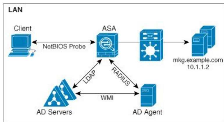
Figure 3: Identity Firewall Components
