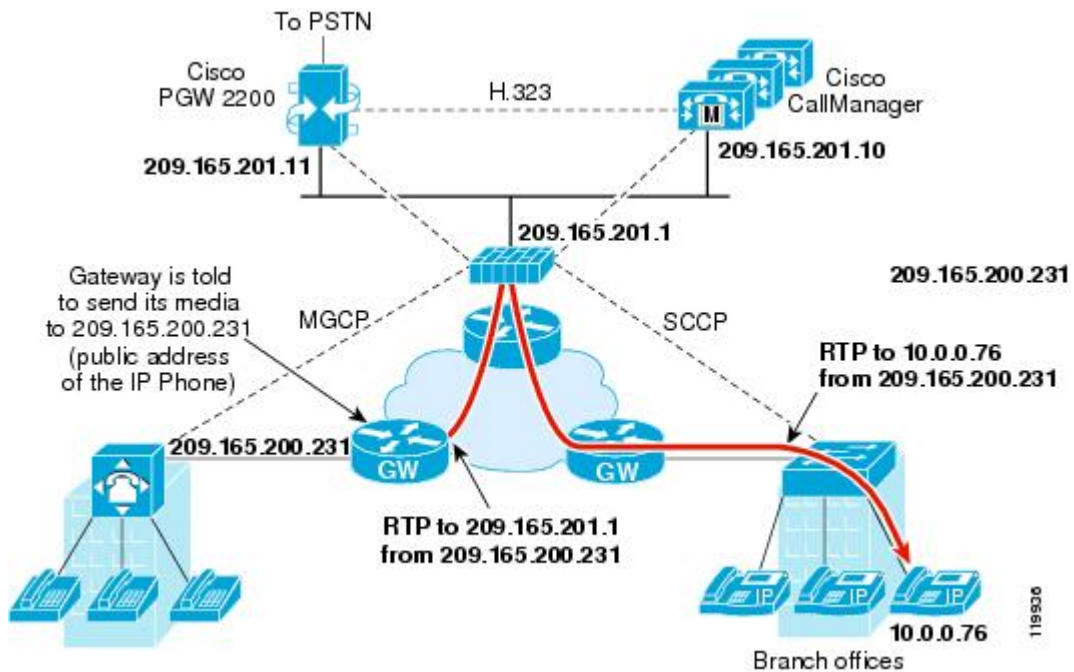
Figure 50: Using NAT with MGCP
