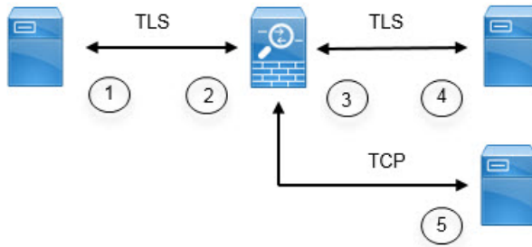
Figure 52: Diameter TLS Inspection
