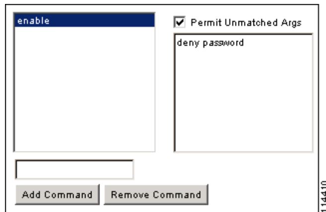
Figure 40-3 Disallowing Arguments
