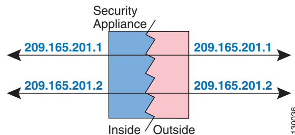
Figure 17-25 Static Identity NAT
