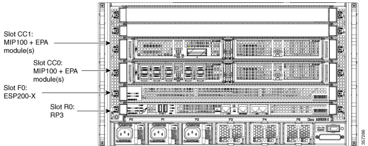
Figure 28: Cisco ASR 1006-X Slots and Modules
