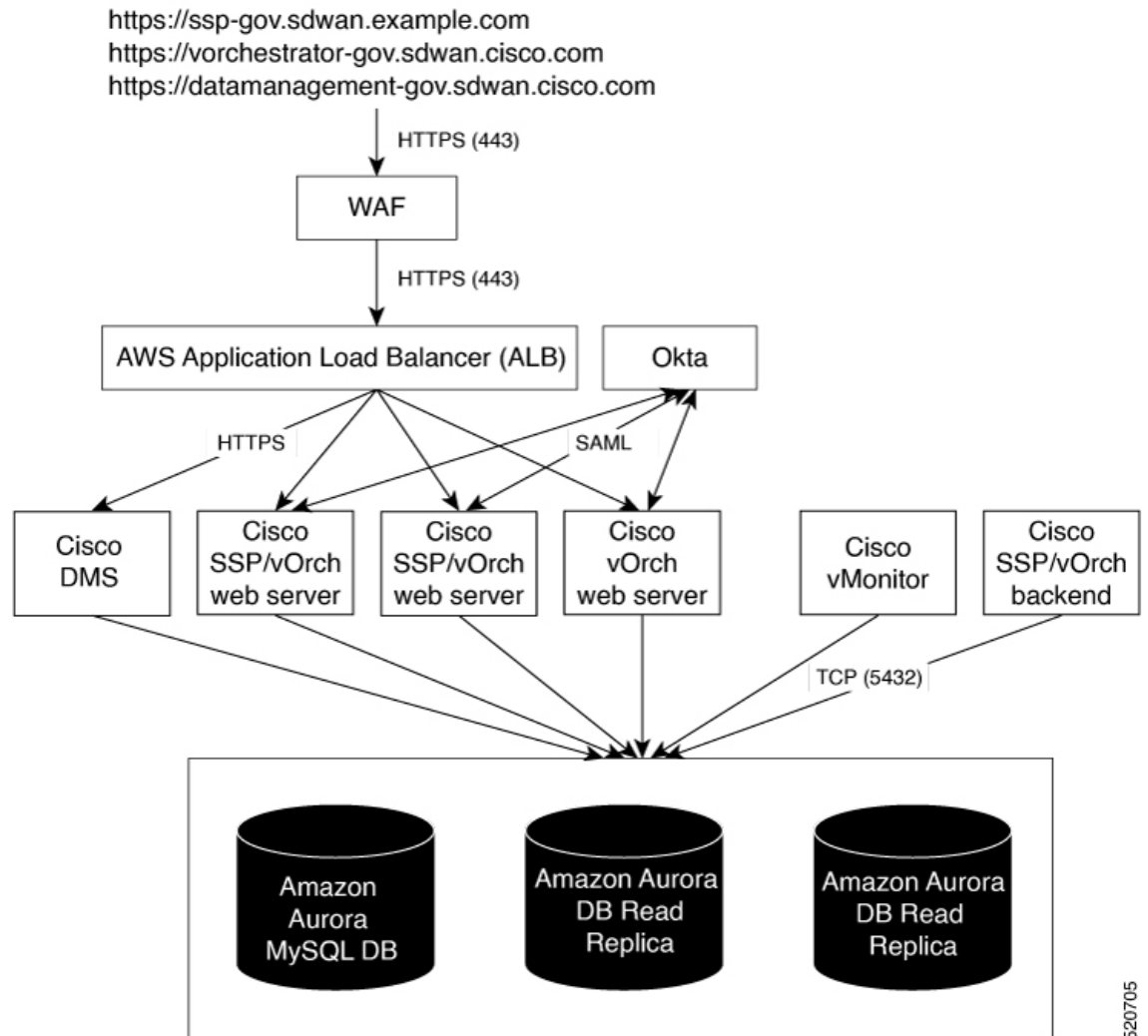
Figure 2: Cisco Catalyst SD-WAN Portal Architecture
