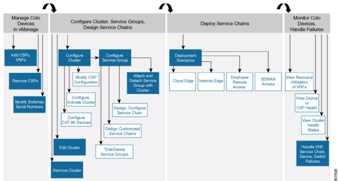
Figure 32: Day-N Workflow
