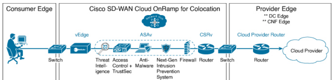
Figure 9: SD-WAN Access Service Chain
