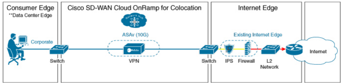
Figure 7: Employee Remote VPN Access Service Chain
