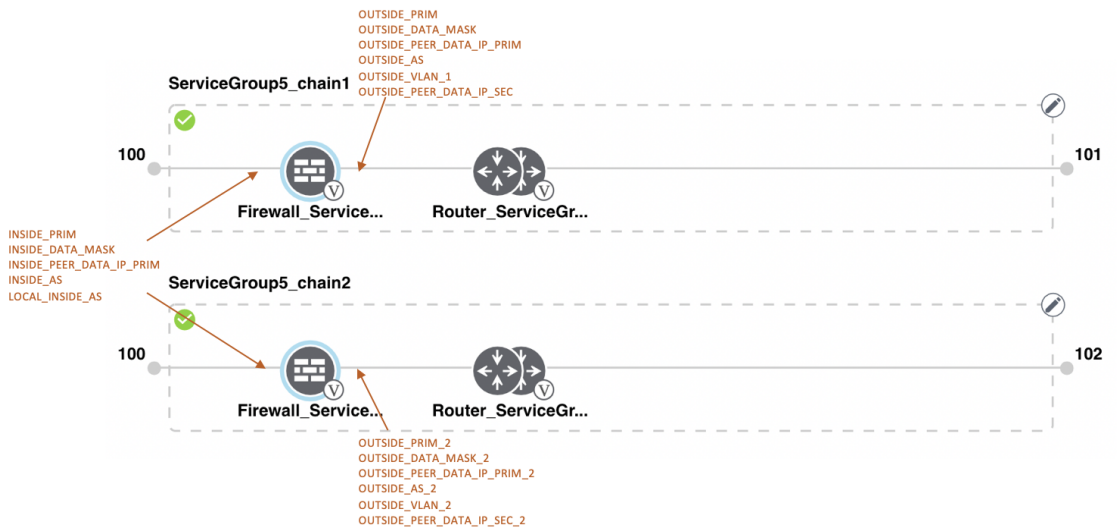
Figure 29: Shared-ASA VNF in First Position
