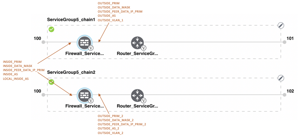
Figure 28: Shared-ASA VNF in First Position
