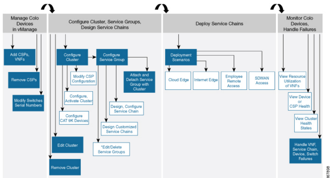
Figure 30: Day-N Workflow
