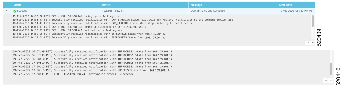
Figure 11: Cluster Activation
