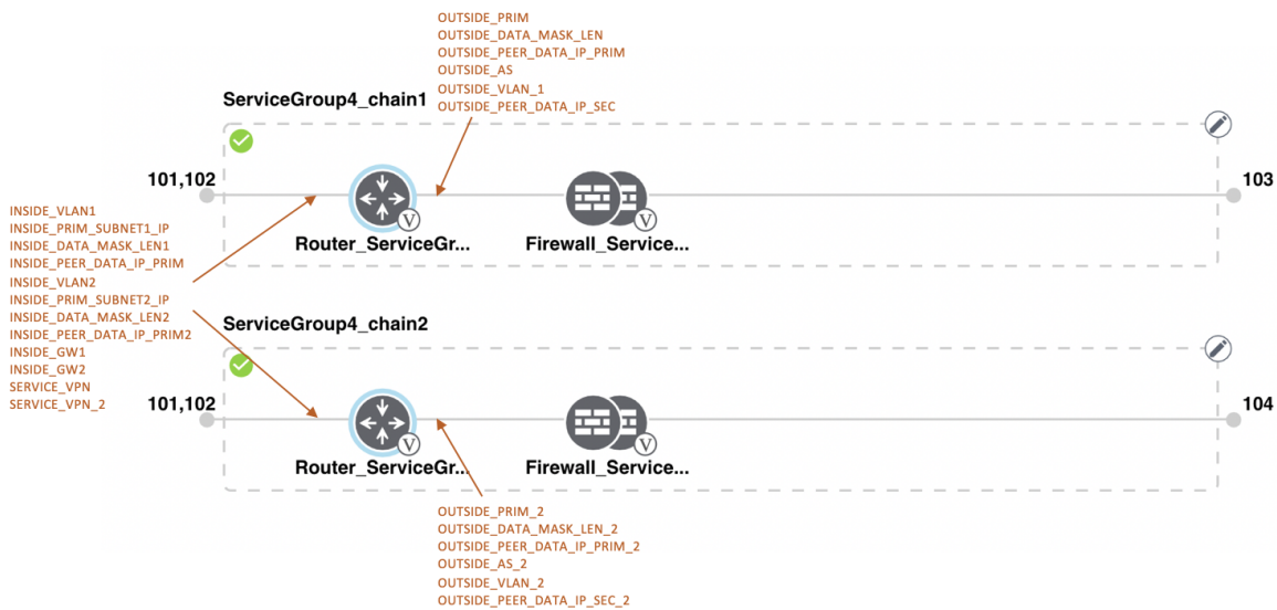
Figure 24: Shared-Cisco CSR1000V VNF in Last Position
