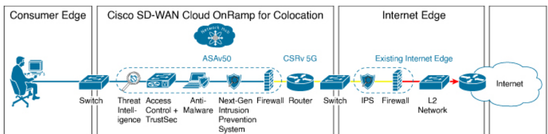
Figure 8: Internet Edge Service Chain
