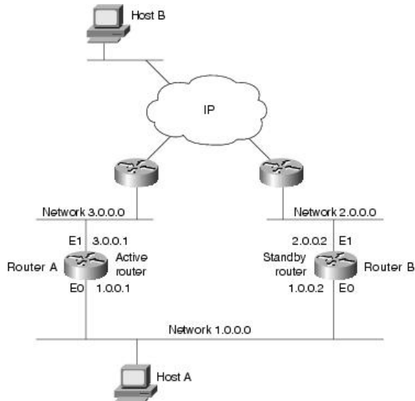
Figure 13: Routers Configured as an HSRP Group
