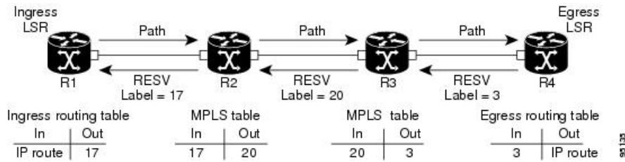
Figure 1: RSVP Operation
