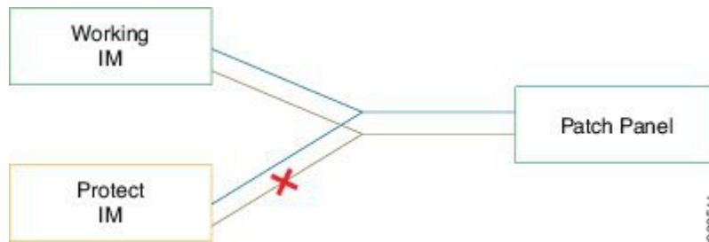
Figure 1: Y Cable
