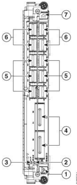
Figure 10: Front Panel of the NCS4K-4H-OPW-QC2 Line Card
