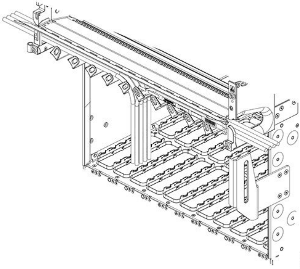
Figure 18: Routing Interface Cables Through the Cable Management Tray
