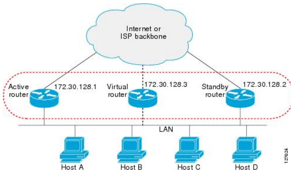
Figure 1: HSRP Topology
