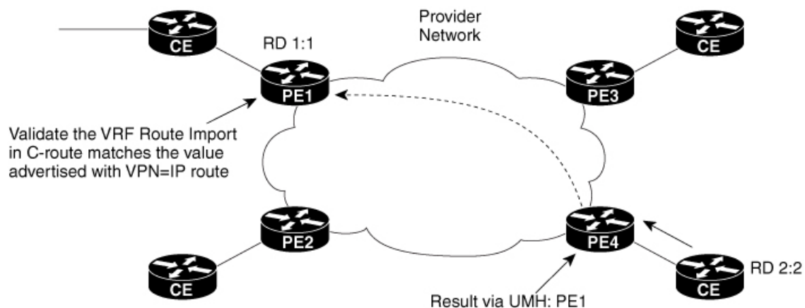
Figure 1: RFC 4761 NLRI
