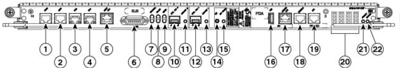
Figure 7: Performance Route Processor Front Panel
