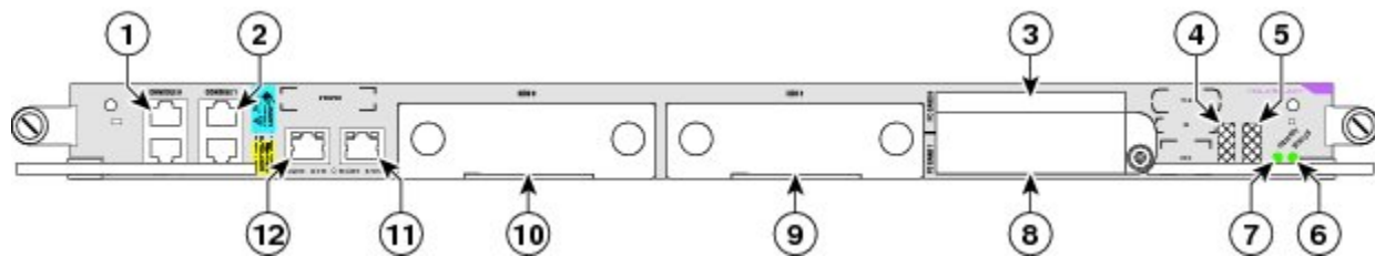
Figure 5: DRP PLIM Front Panel
