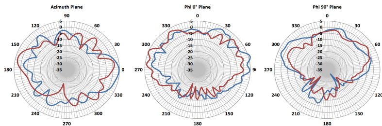
Figure 15: 5875 MHz WLAN Antenna Radiation Patterns
