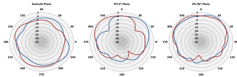
Figure 7: 1710 MHz Cellular Antenna Radiation Patterns
