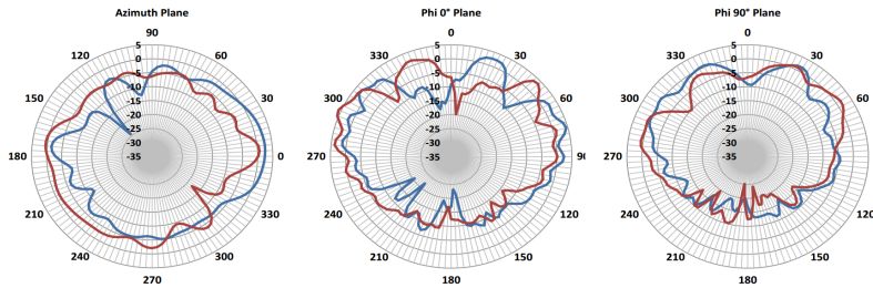
Figure 14: 5275 MHz WLAN Antenna Radiation Patterns
