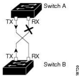
Figure 6: Unidirectional Link
