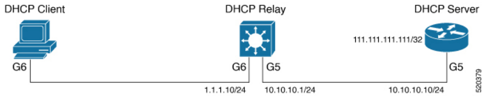
Figure 5: Topology Showing DHCP Client with GigabitEthernet Interface
