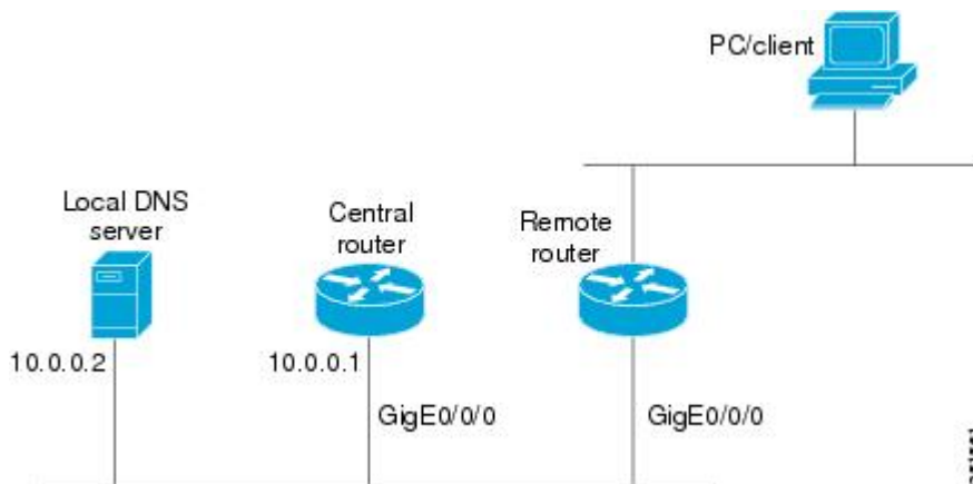
Figure 2: DHCP Example Network Topology
