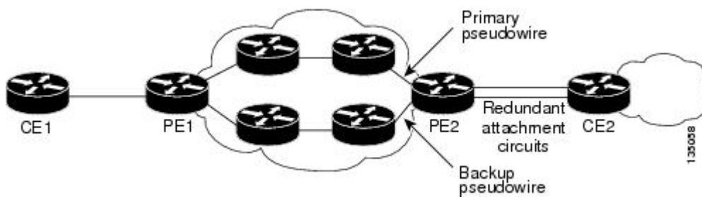
Figure 3: Pseudowire Redundancy
