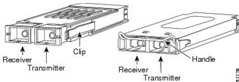
Figure 1: GBICs with Clips (Left) and with a Handle (Right)
